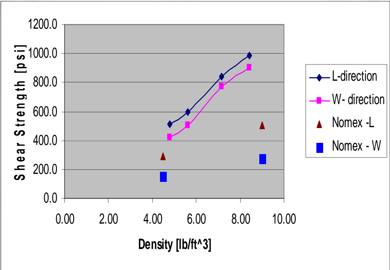
Ti Core Shear Strength Compared to Nomex Core
